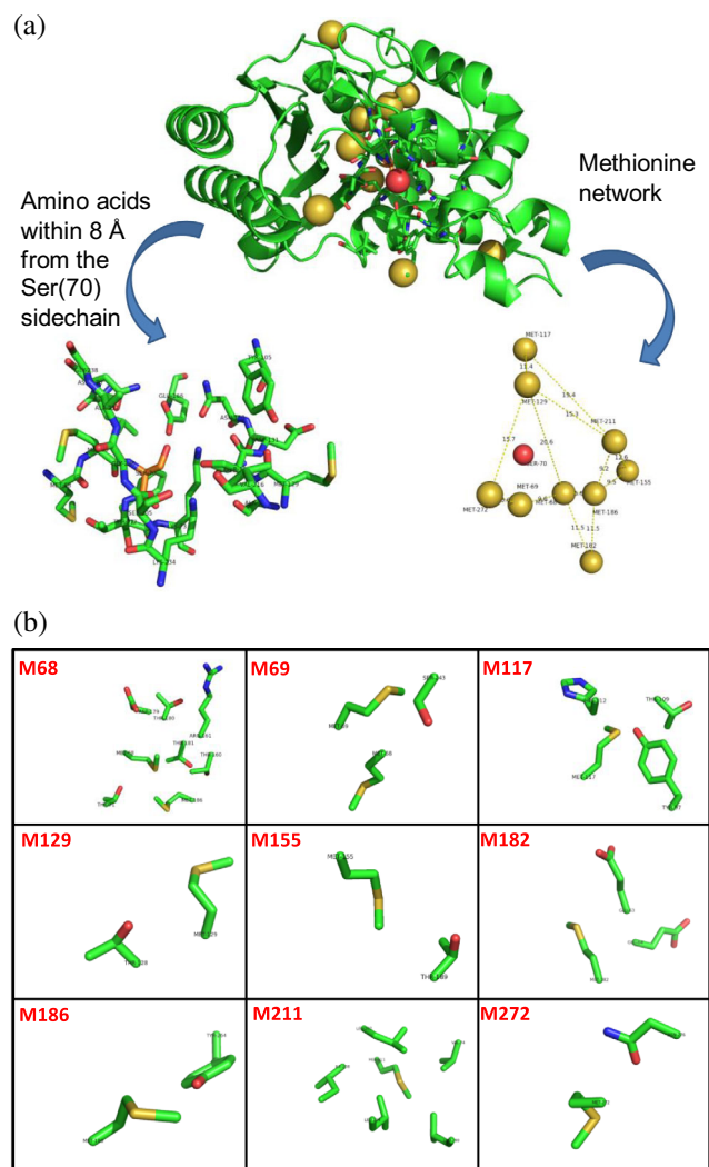
FIGURE 5 Structure of the TEM-1 \beta -lactamase (PDB id: 1zq4) highlighting the putative metal ion binding sites. (a) Coordinating amino acids with potential donor groups for metal ion coordination within 8 Å surroundings of the S70 sidechain and the network of methionines with distances between the sulfur donor atoms. (b) Amino acids containing further putative coordinating donor atoms in the 5 Å surroundings of each methionine sulfur.
